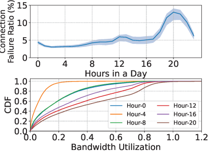
Figure 5: Change in core indicators of the edge network within a day
