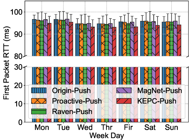
Figure 25: Evaluation of the average first packet RTT
